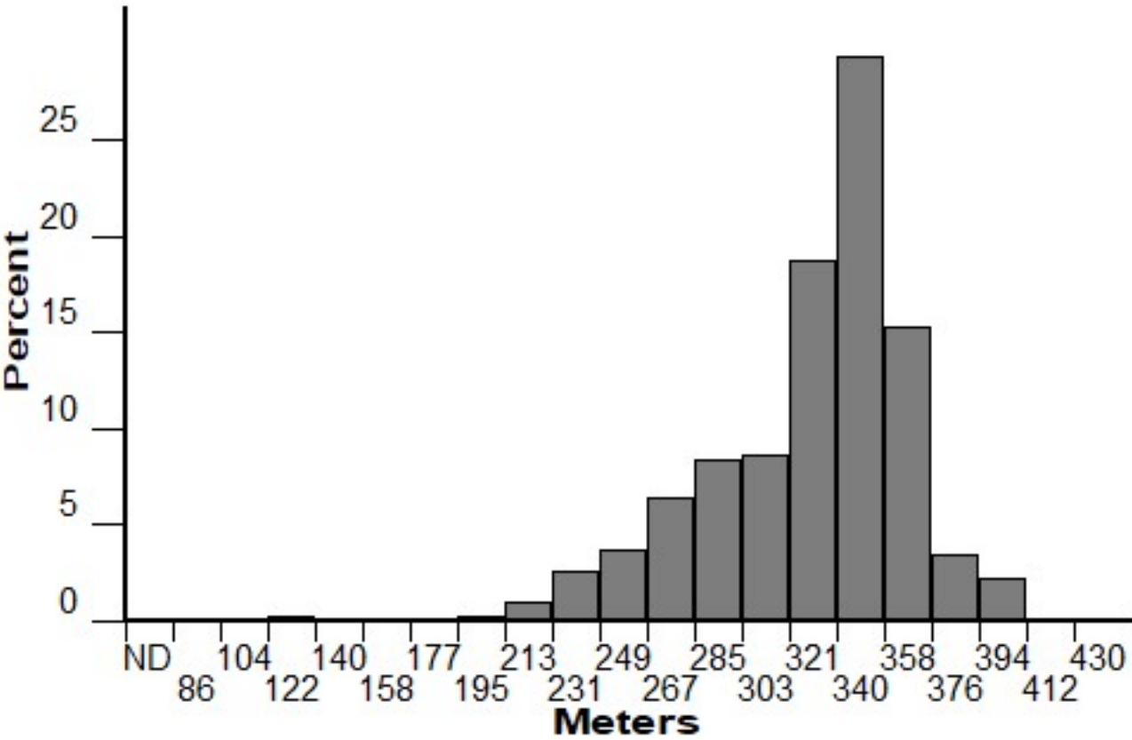
Elevation (FM 185)
