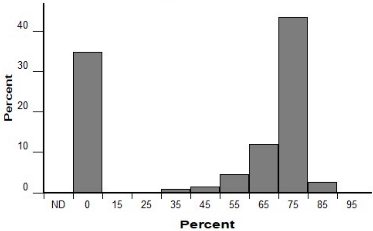
Canopy Cover
