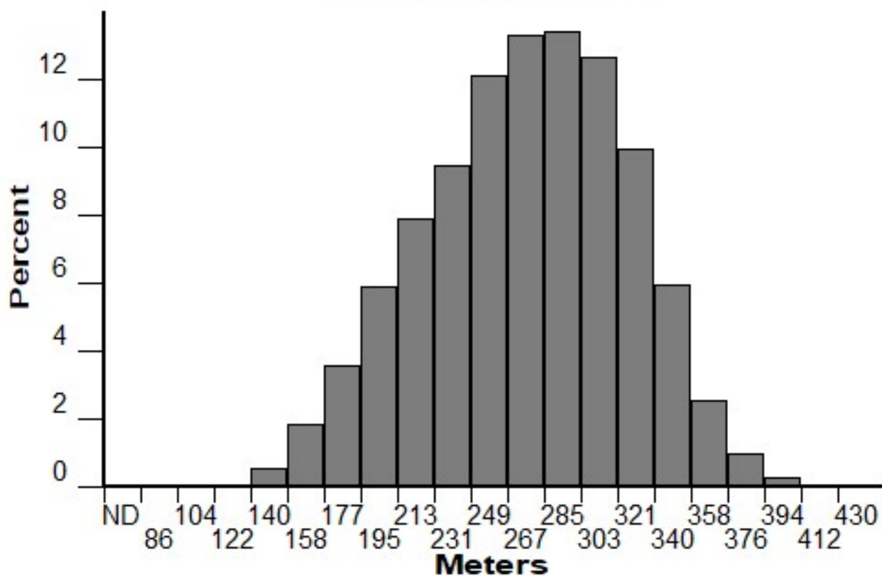
Elevation (FM 188)
